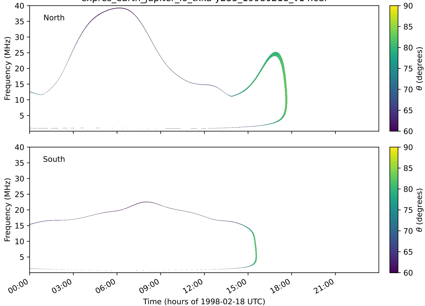
expres_earth_jupiter_io_txka-y235_19980218_v14.cdf
