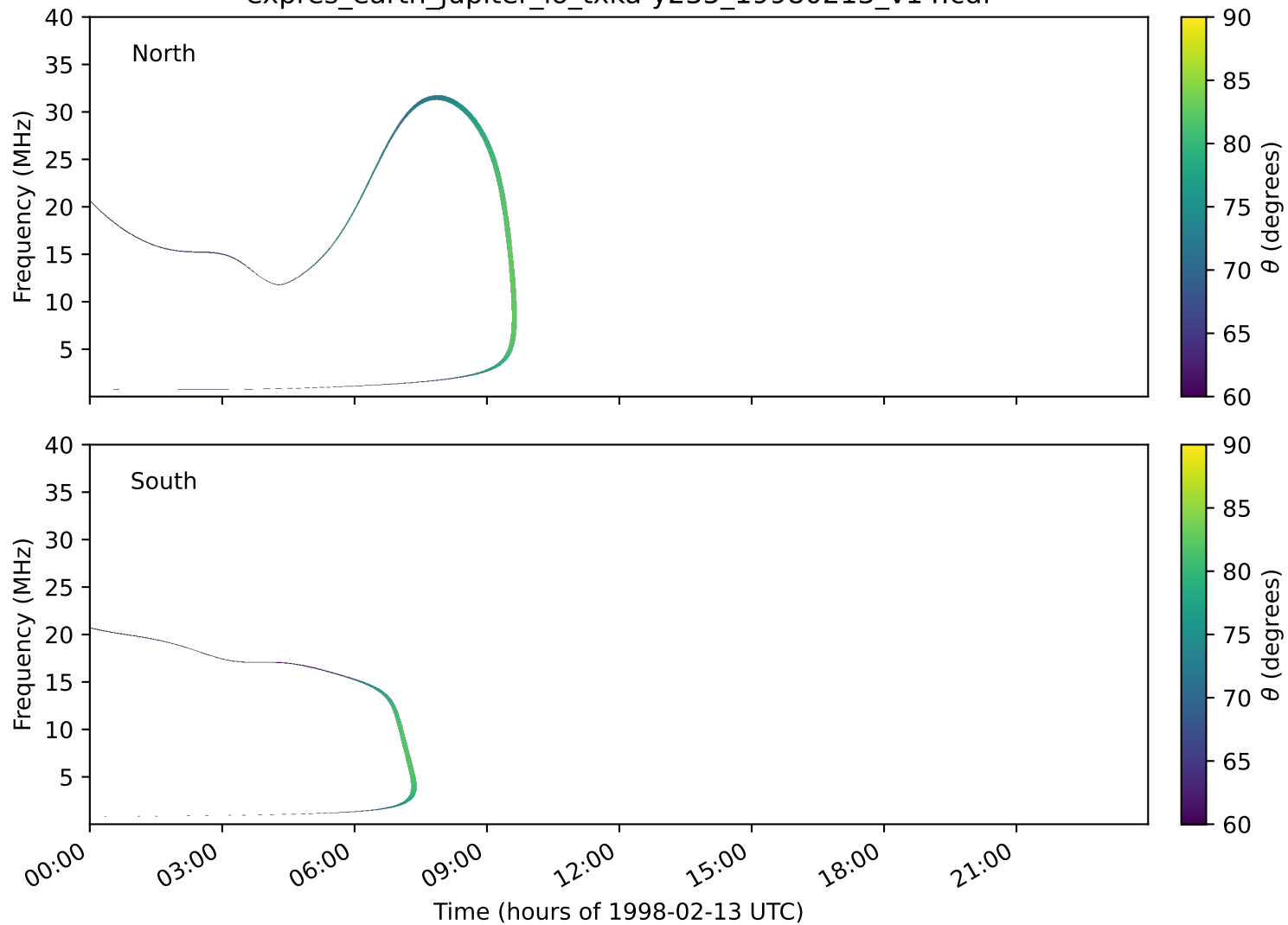
expres_earth_jupiter_io_txka-y235_19980213_v14.cdf
