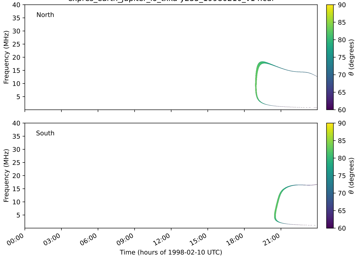
expres_earth_jupiter_io_txka-y235_19980210_v14.cdf
