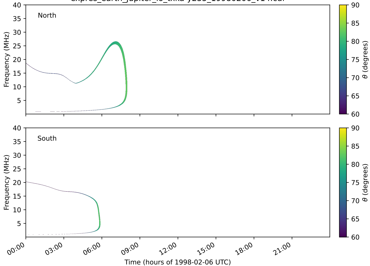
expres_earth_jupiter_io_txka-y235_19980206_v14.cdf
