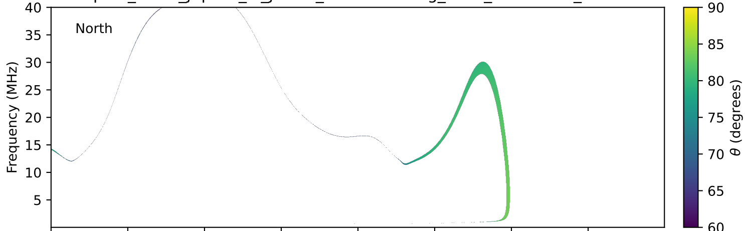
expres_earth_jupiter_io_jrm33_lossc-wid1deg_3kev_19980218_v11.cdf
