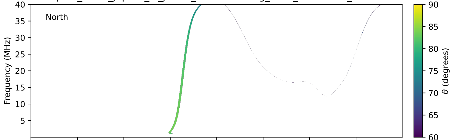
expres_earth_jupiter_io_jrm33_lossc-wid1deg_3kev_19980214_v11.cdf
