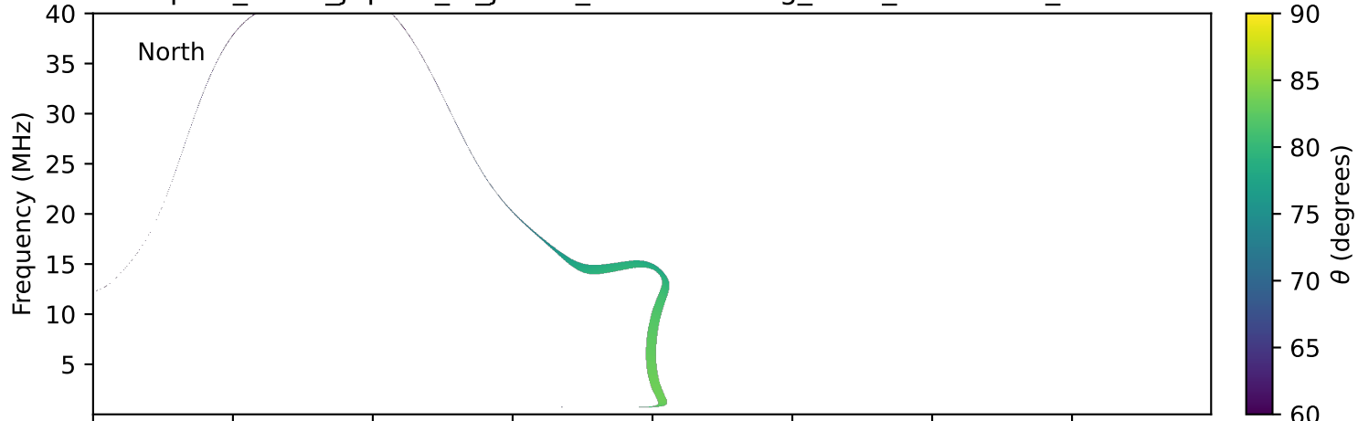
expres_earth_jupiter_io_jrm33_lossc-wid1deg_3kev_19980204_v11.cdf
