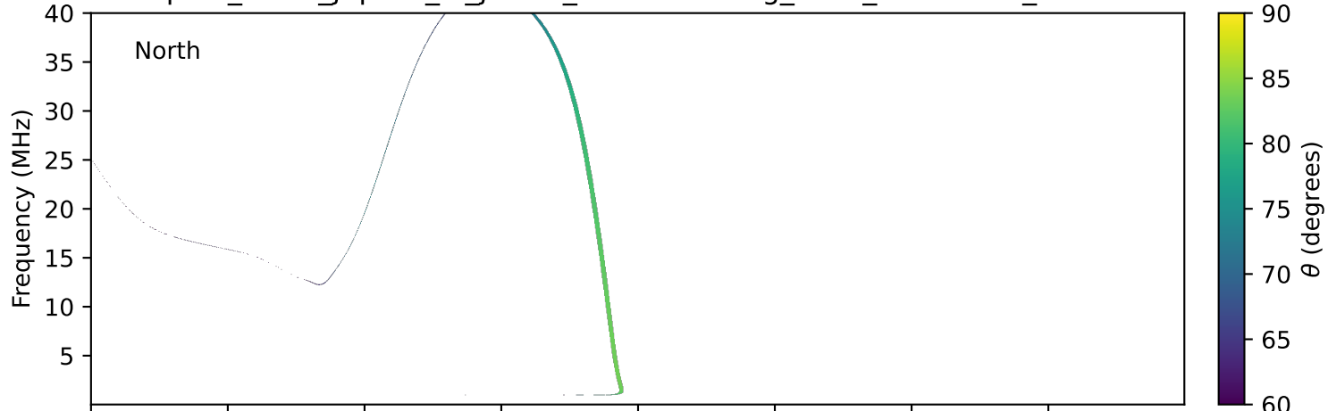
expres_earth_jupiter_io_jrm09_lossc-wid1deg_3kev_19980220_v11.cdf
