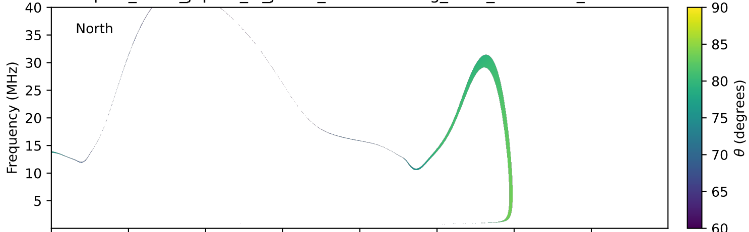
expres_earth_jupiter_io_jrm09_lossc-wid1deg_3kev_19980218_v11.cdf
