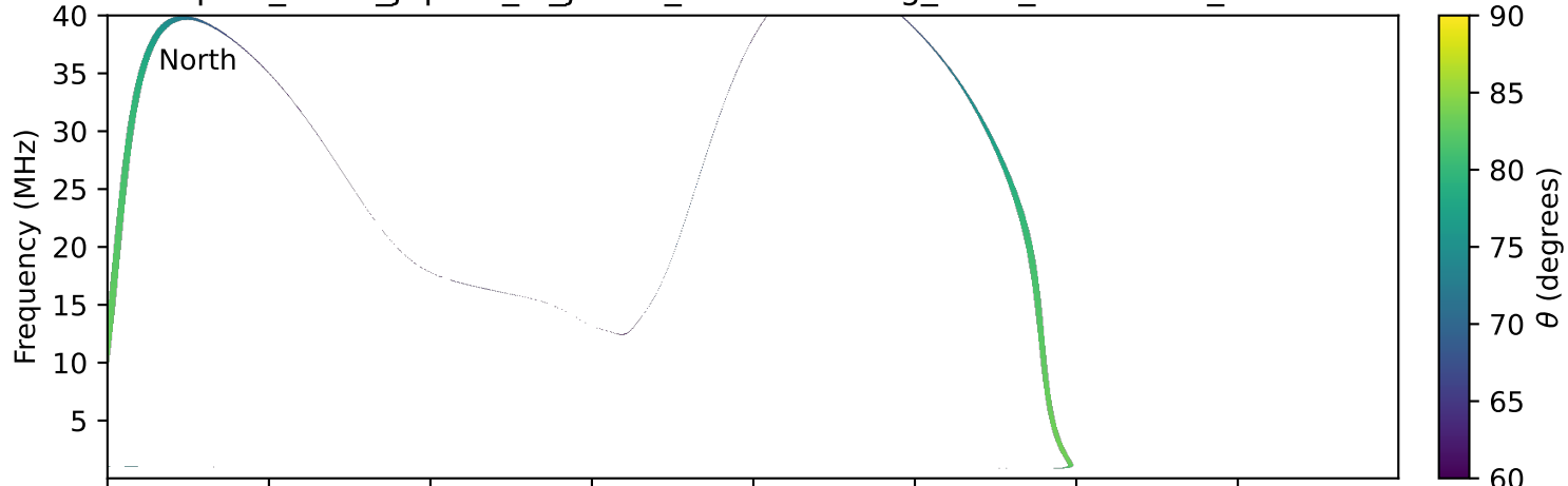
expres_earth_jupiter_io_jrm09_lossc-wid1deg_3kev_19980202_v11.cdf
