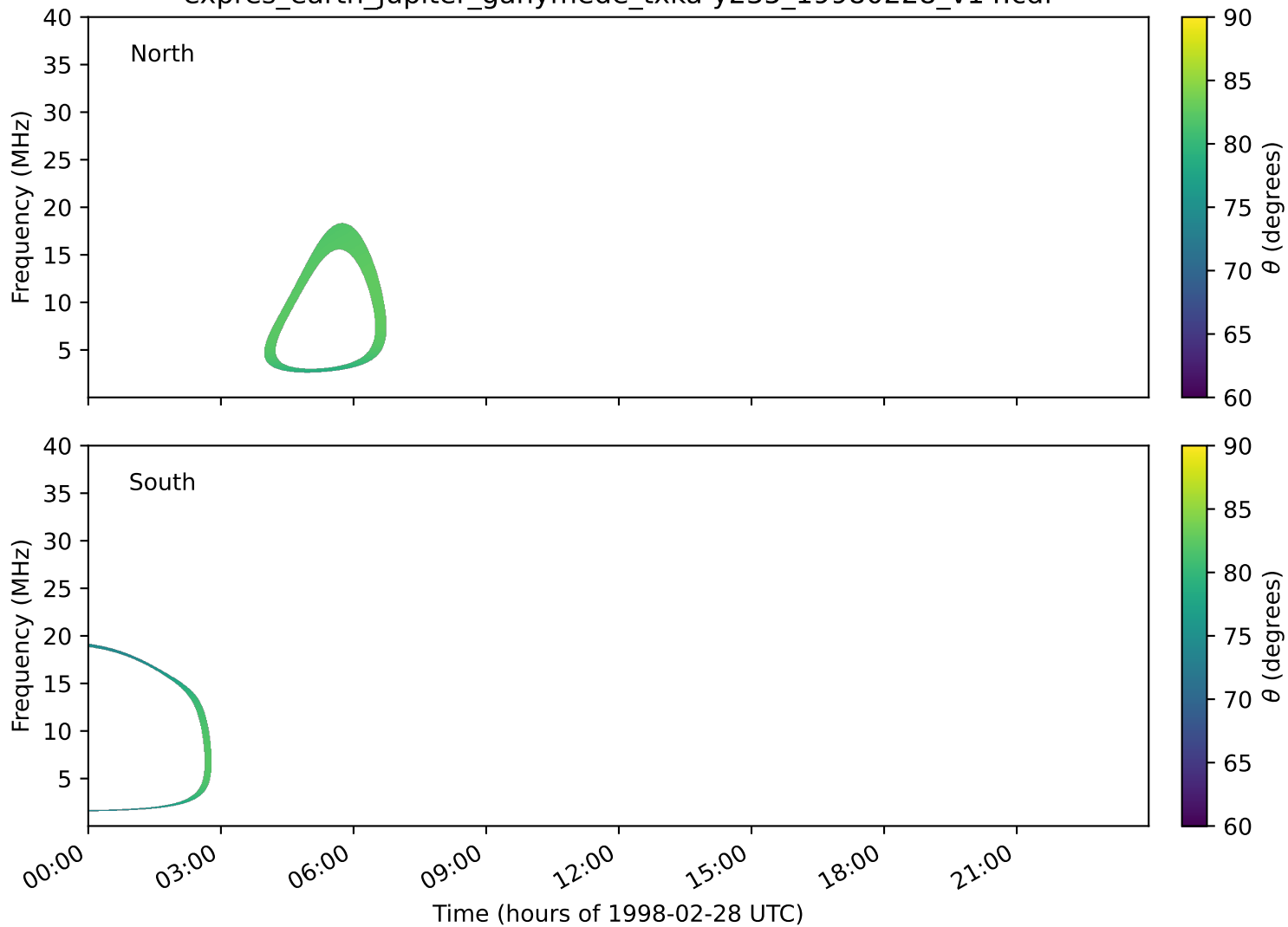
expres_earth_jupiter_ganymede_txka-y235_19980228_v14.cdf
