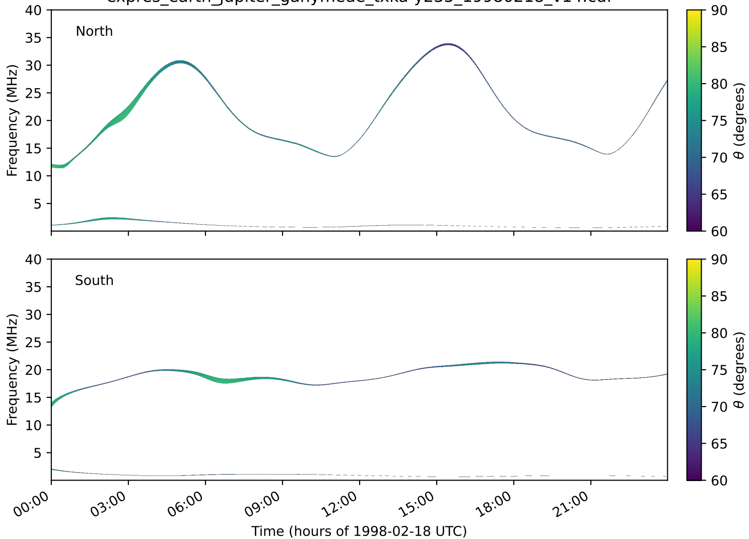
expres_earth_jupiter_ganymede_txka-y235_19980218_v14.cdf
