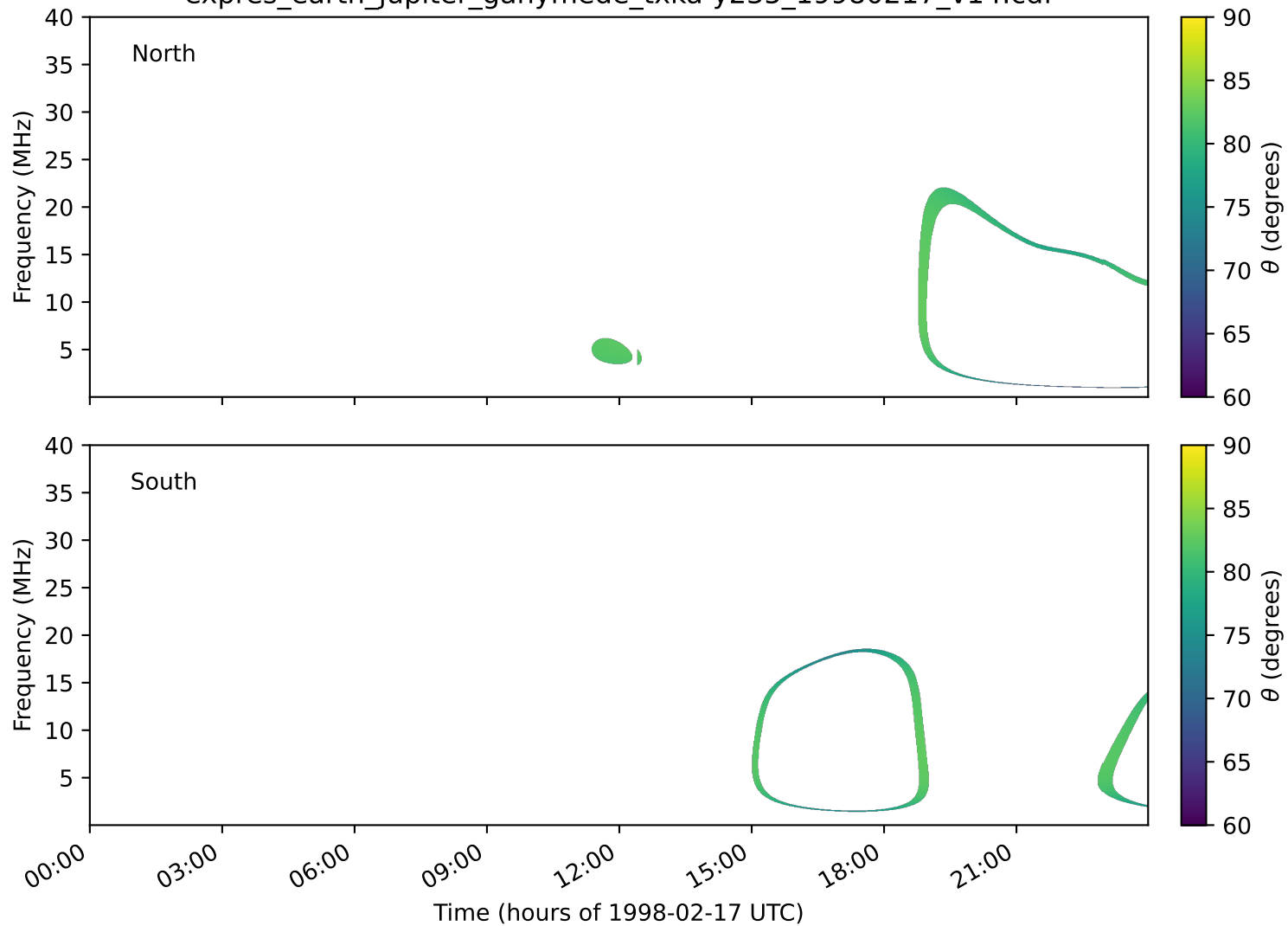
expres_earth_jupiter_ganymede_txka-y235_19980217_v14.cdf
