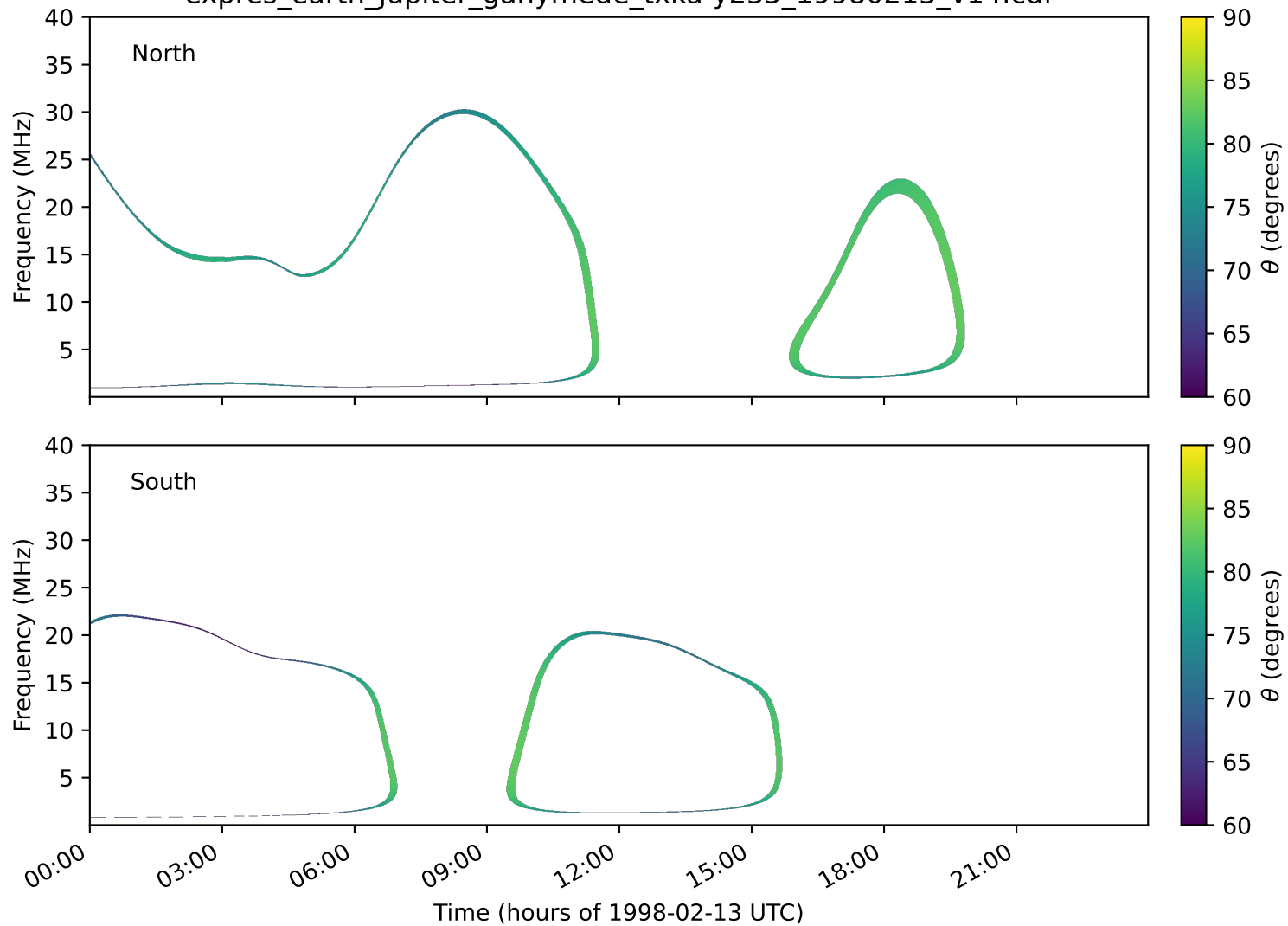
expres_earth_jupiter_ganymede_txka-y235_19980213_v14.cdf
