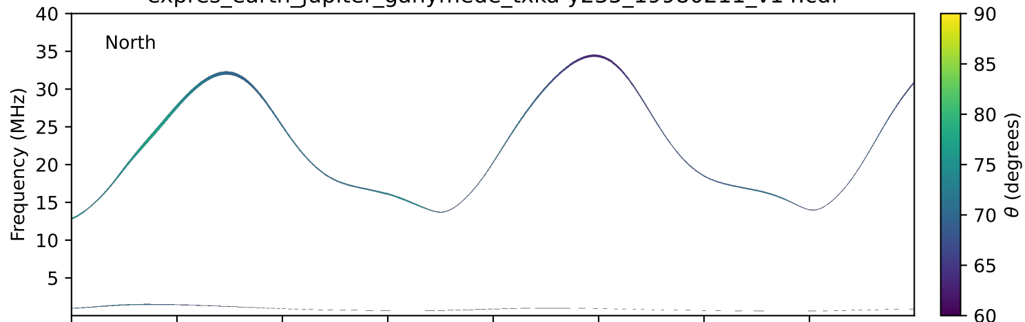
expres_earth_jupiter_ganymede_txka-y235_19980211_v14.cdf
