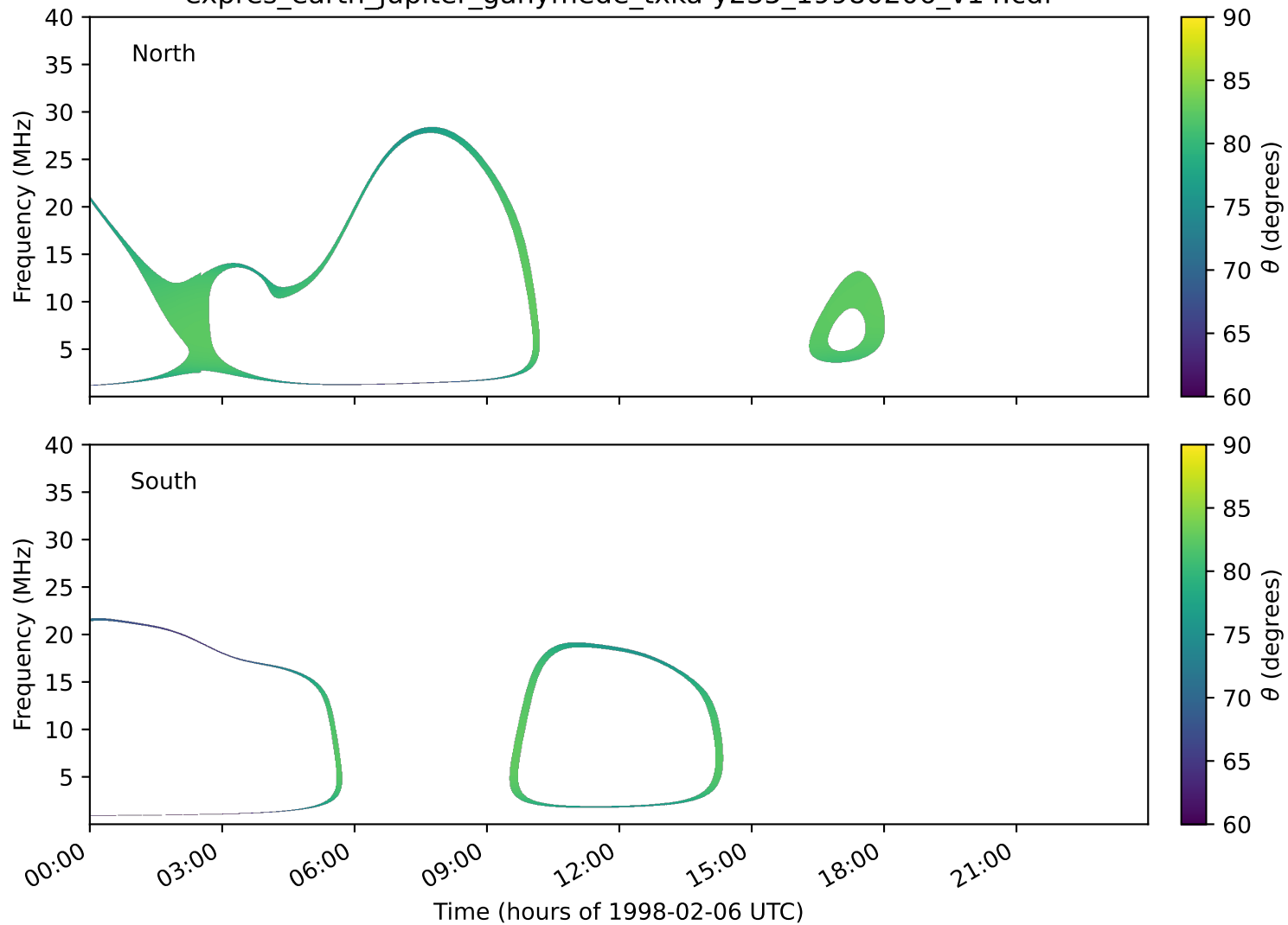
expres_earth_jupiter_ganymede_txka-y235_19980206_v14.cdf
