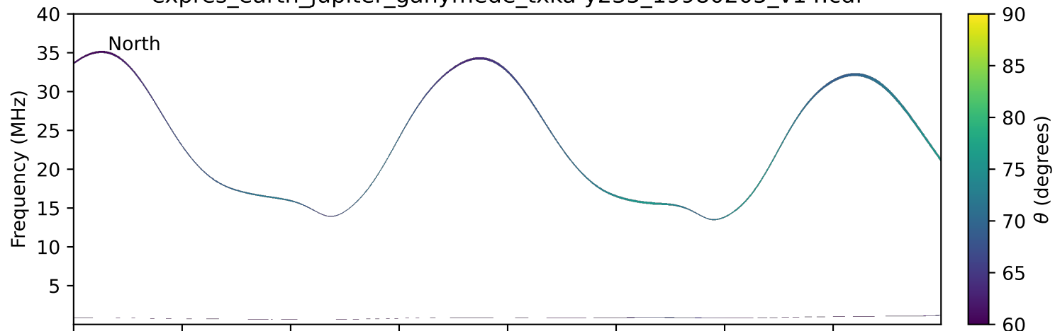
expres_earth_jupiter_ganymede_txka-y235_19980205_v14.cdf
