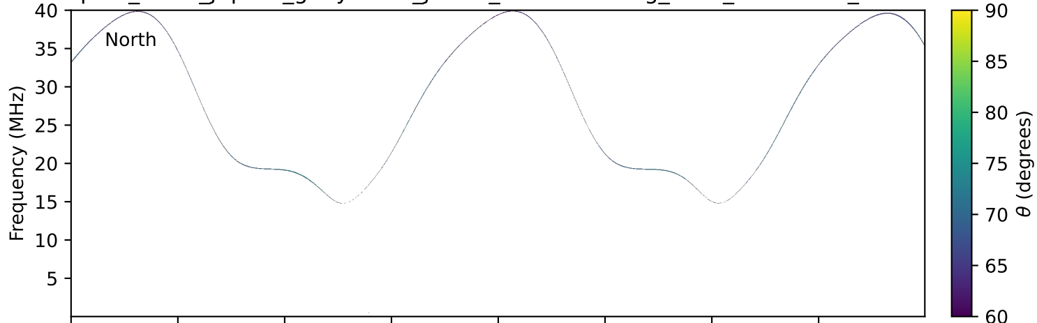
expres_earth_jupiter_ganymede_jrm33_lossc-wid1deg_3kev_19980219_v11.cdf
