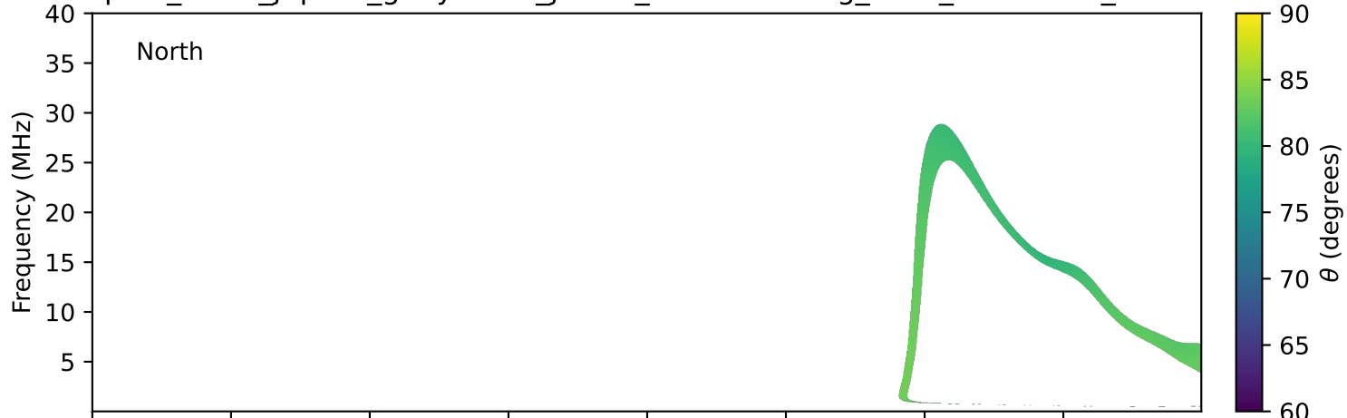
expres_earth_jupiter_ganymede_jrm33_lossc-wid1deg_3kev_19980210_v11.cdf
