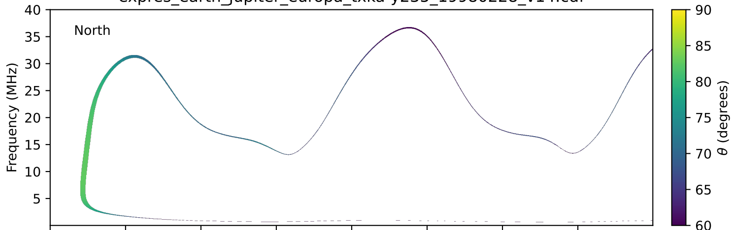
expres_earth_jupiter_europa_txka-y235_19980228_v14.cdf
