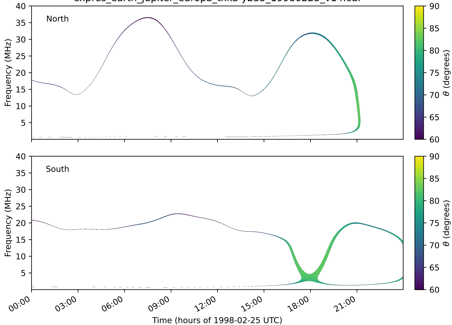
expres_earth_jupiter_europa_txka-y235_19980225_v14.cdf
