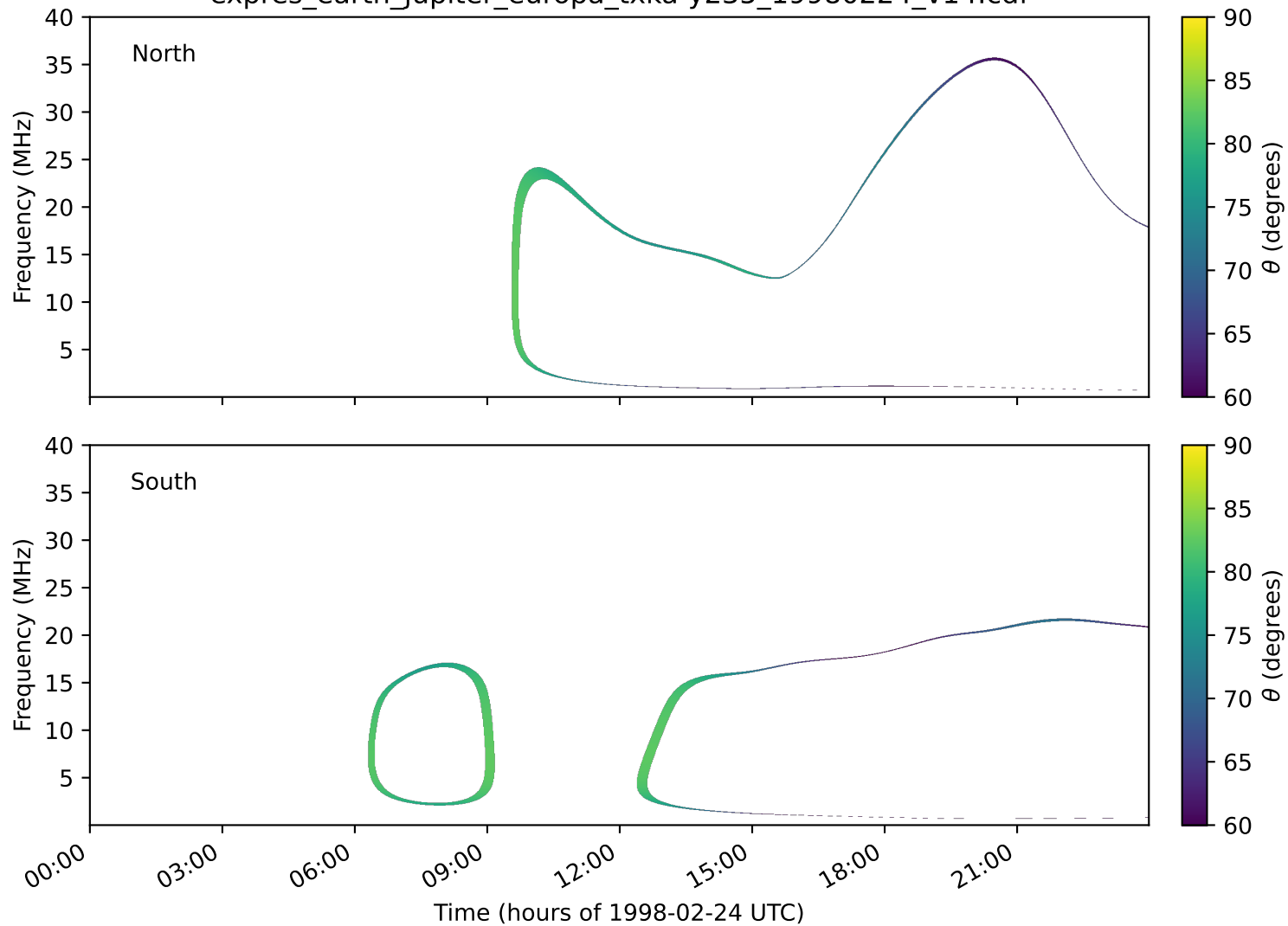
expres_earth_jupiter_europa_txka-y235_19980224_v14.cdf
