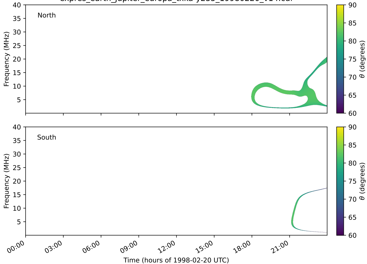
expres_earth_jupiter_europa_txka-y235_19980220_v14.cdf
