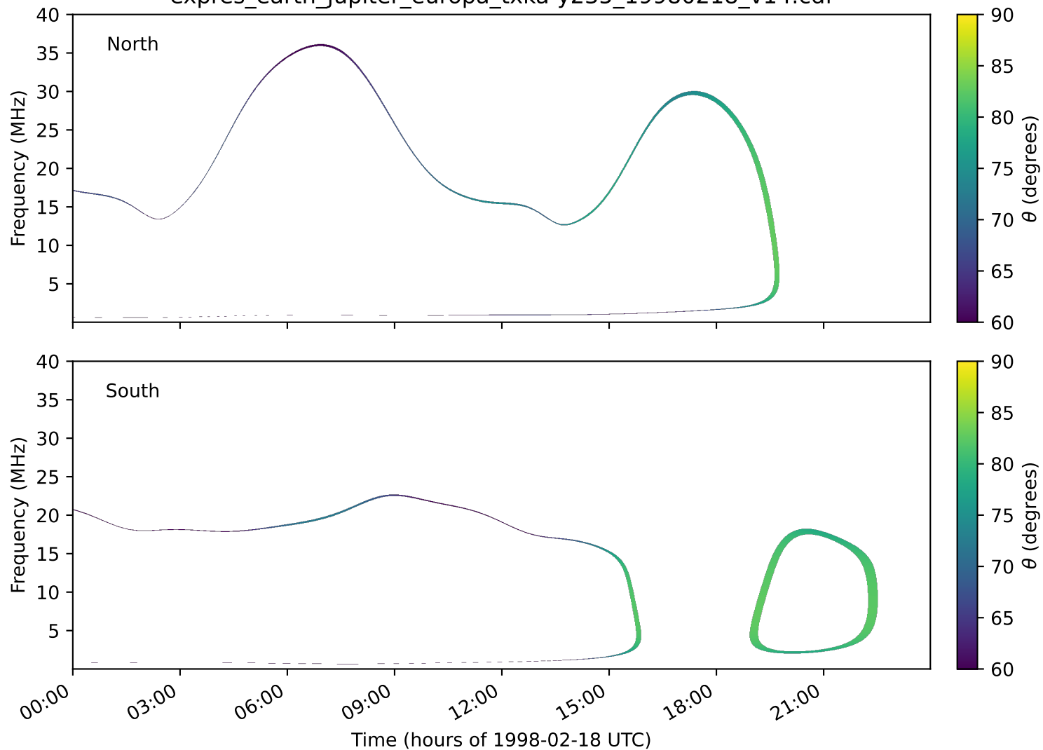
expres_earth_jupiter_europa_txka-y235_19980218_v14.cdf
