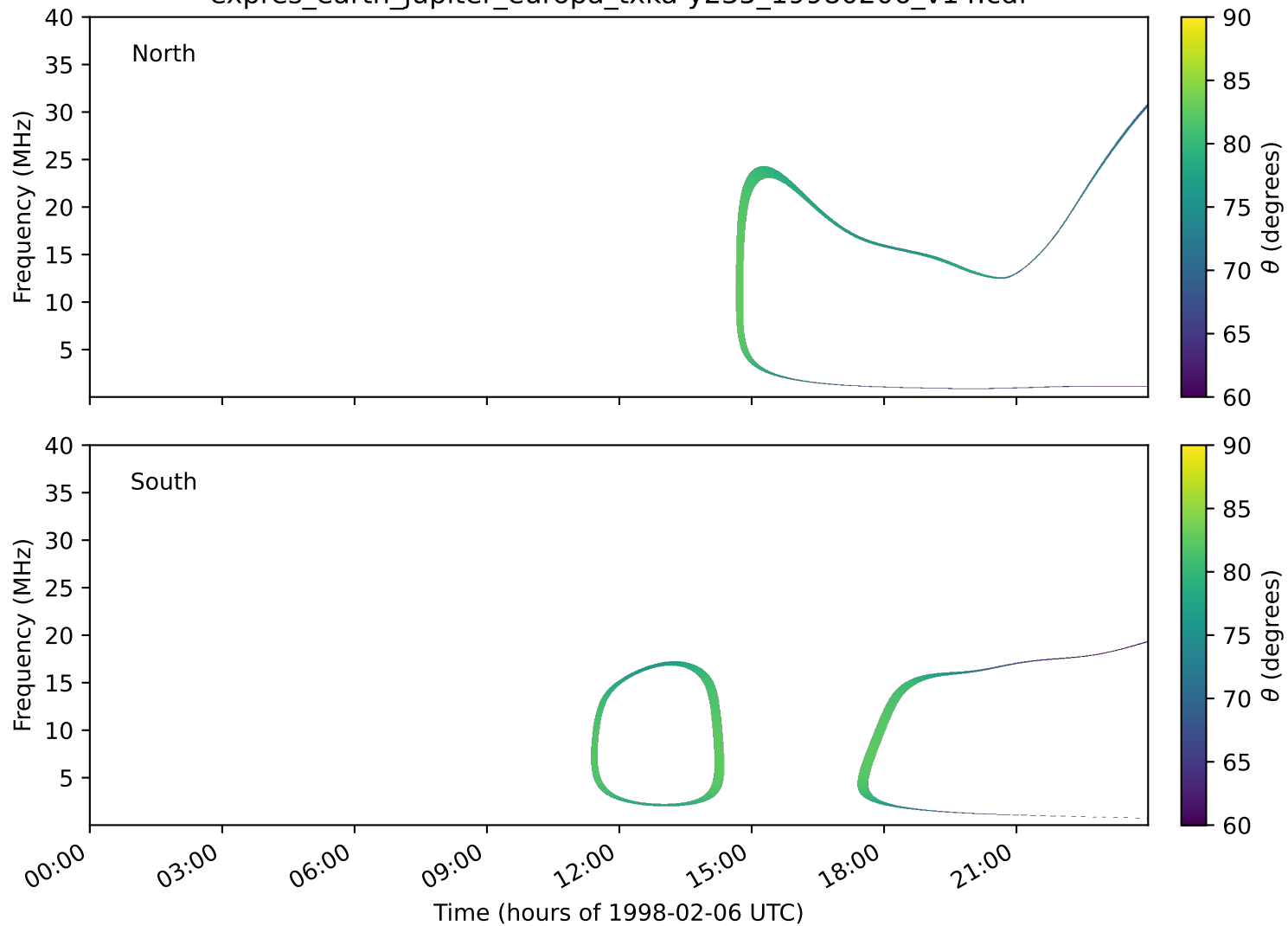
expres_earth_jupiter_europa_txka-y235_19980206_v14.cdf
