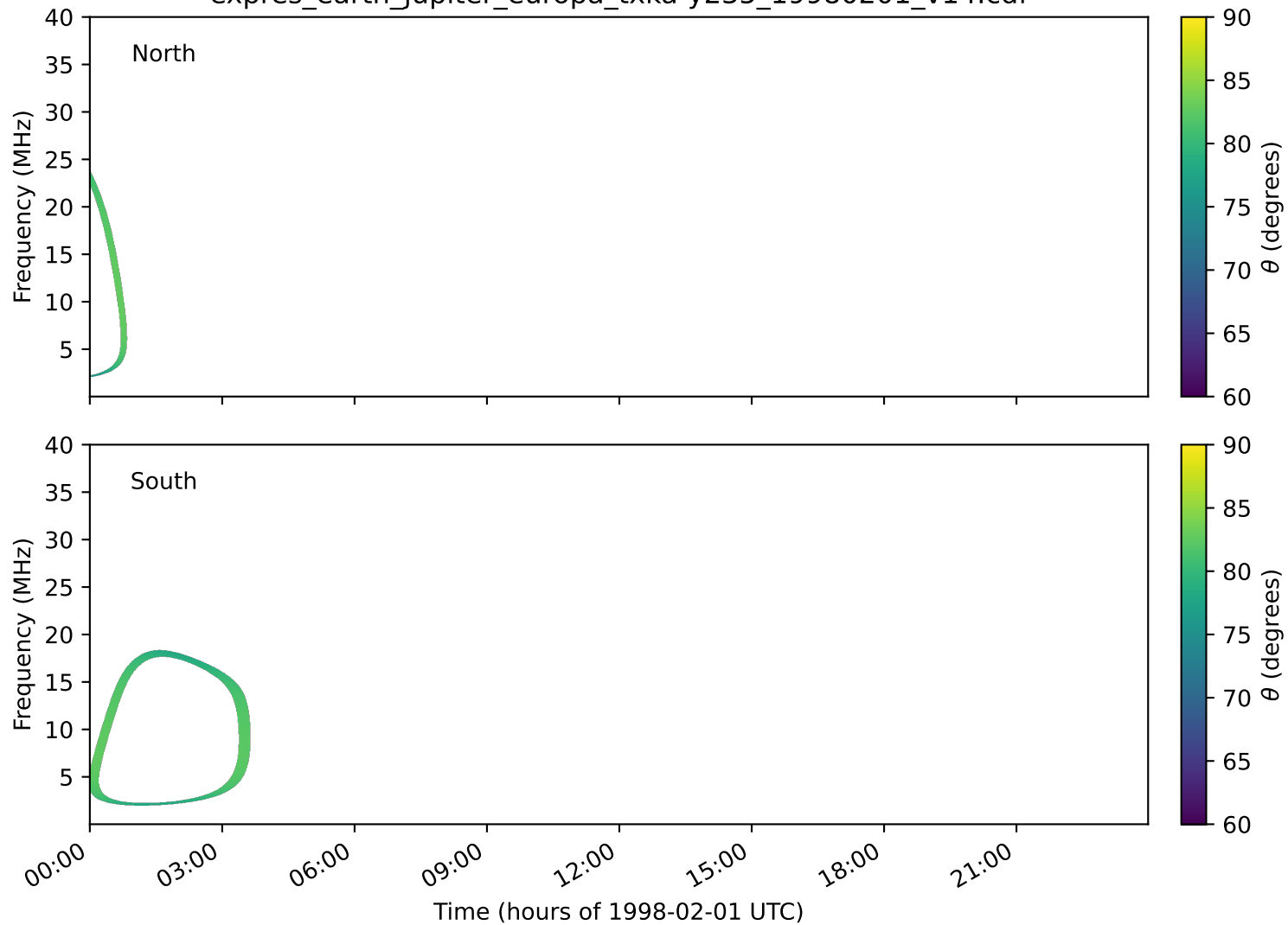
expres_earth_jupiter_europa_txka-y235_19980201_v14.cdf
