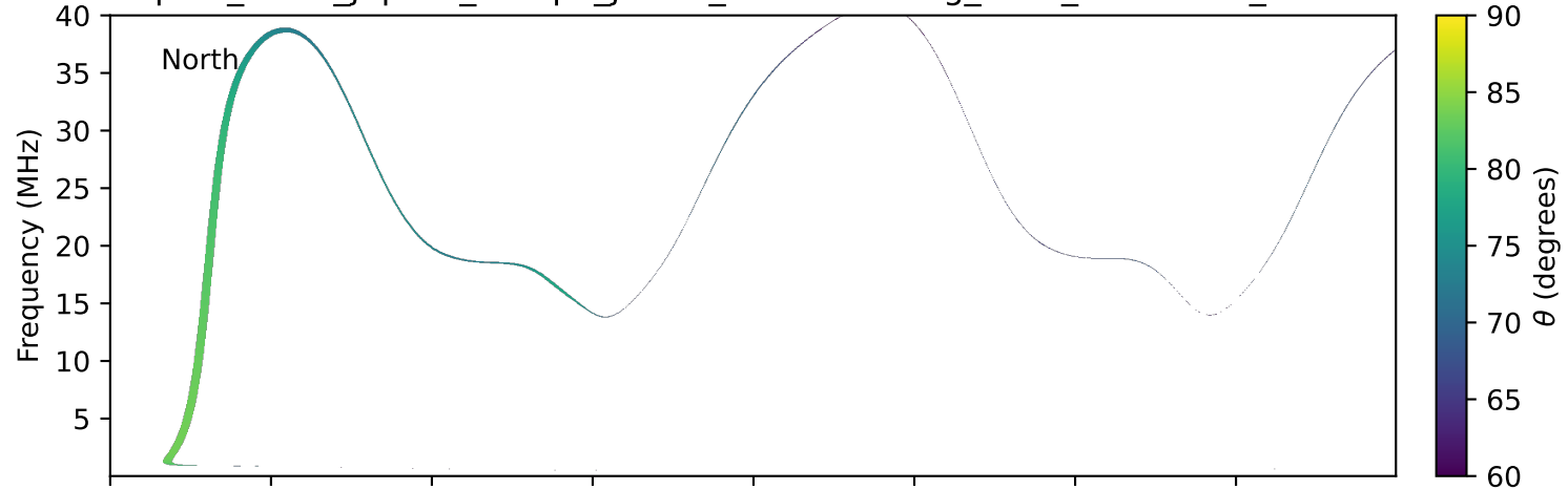
expres_earth_jupiter_europa_jrm33_lossc-wid1deg_3kev_19980228_v11.cdf
