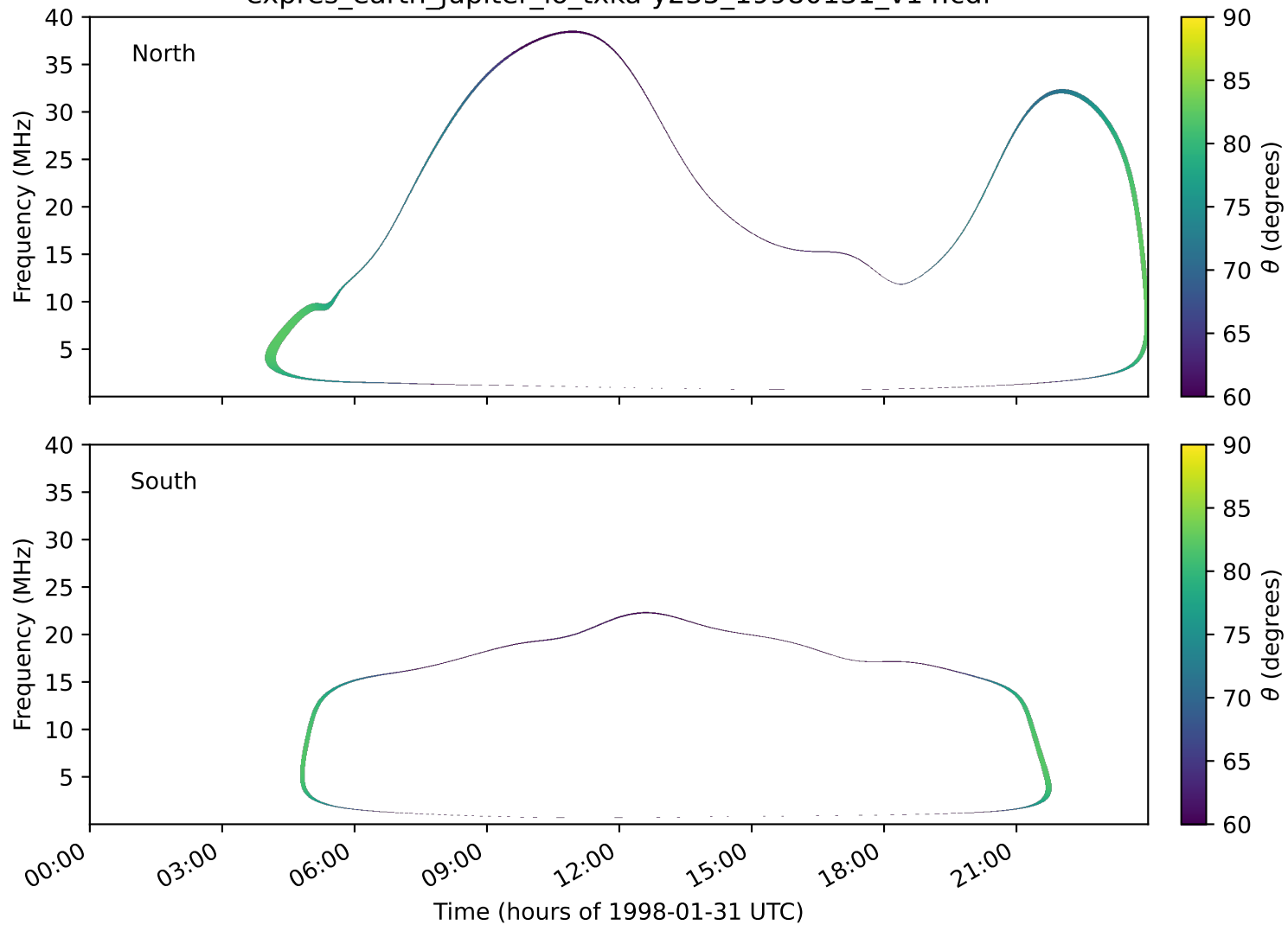
expres_earth_jupiter_io_txka-y235_19980131_v14.cdf
