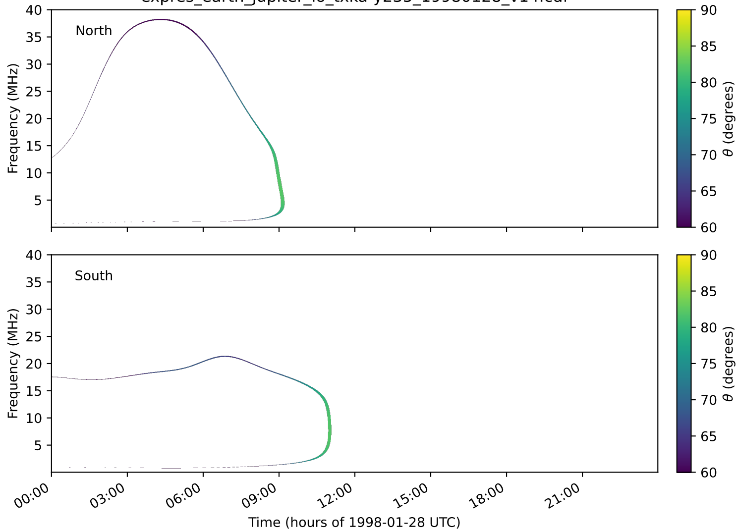
expres_earth_jupiter_io_txka-y235_19980128_v14.cdf
