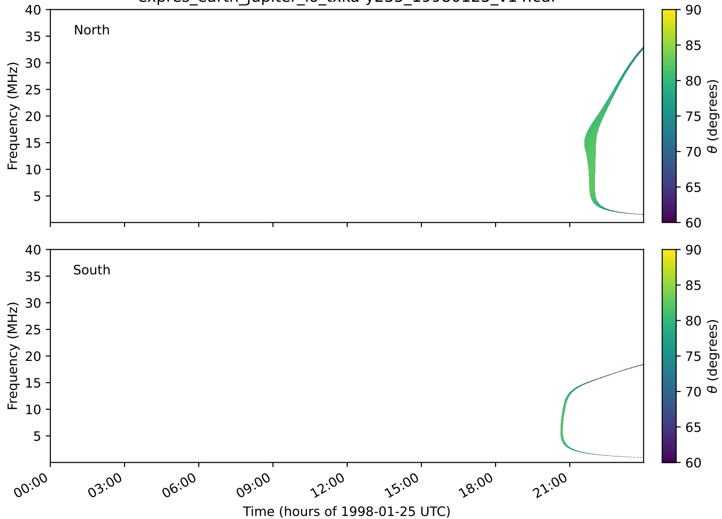
expres_earth_jupiter_io_txka-y235_19980125_v14.cdf
