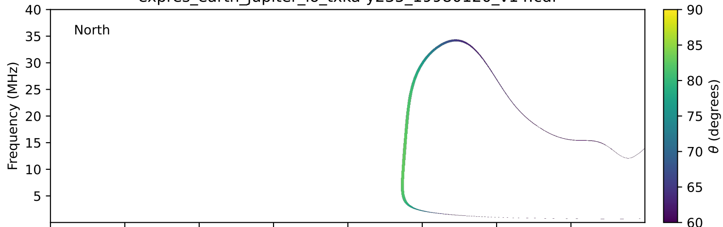
expres_earth_jupiter_io_txka-y235_19980120_v14.cdf
