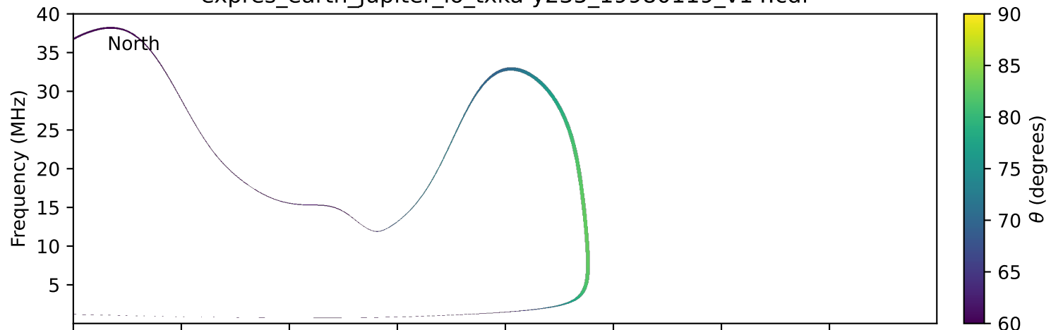
expres_earth_jupiter_io_txka-y235_19980119_v14.cdf
