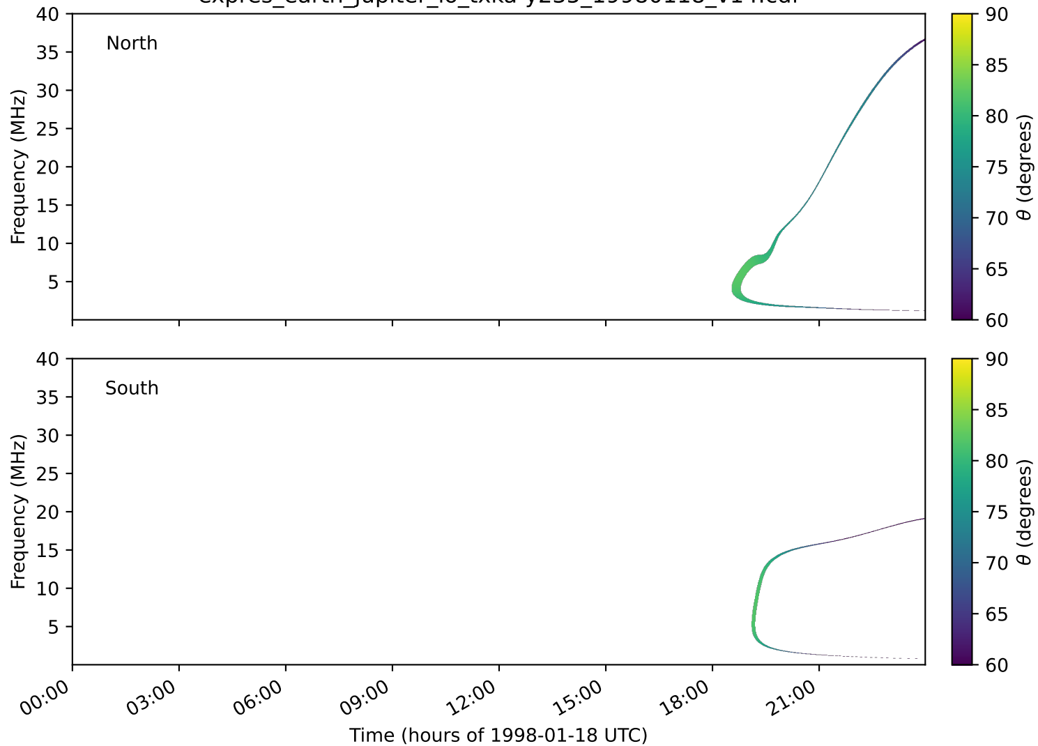
expres_earth_jupiter_io_txka-y235_19980118_v14.cdf
