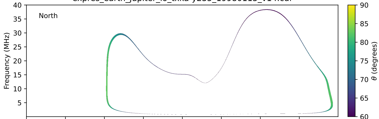
expres_earth_jupiter_io_txka-y235_19980115_v14.cdf
