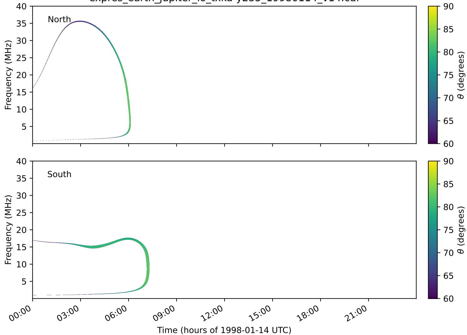
expres_earth_jupiter_io_txka-y235_19980114_v14.cdf
