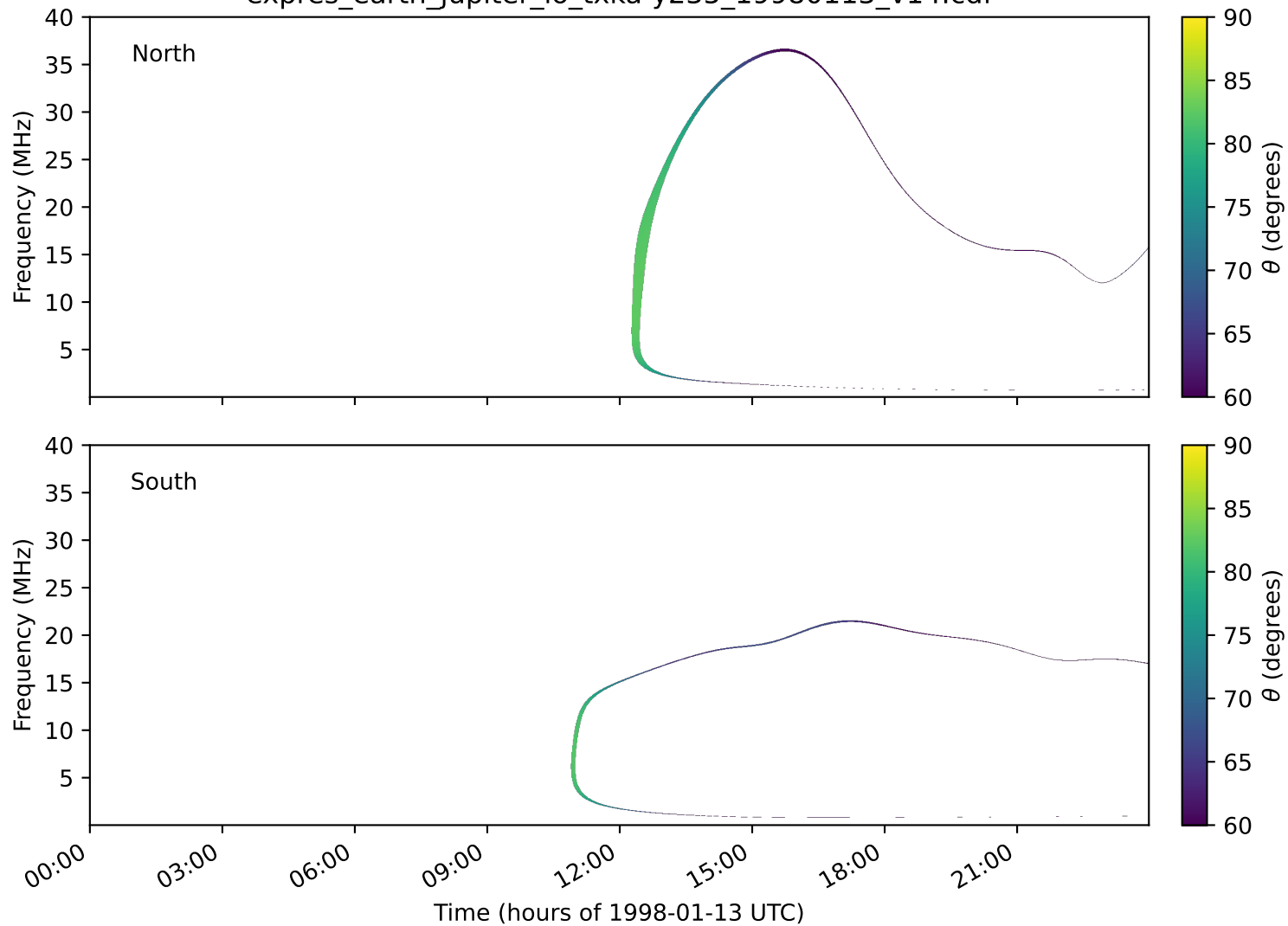
expres_earth_jupiter_io_txka-y235_19980113_v14.cdf
