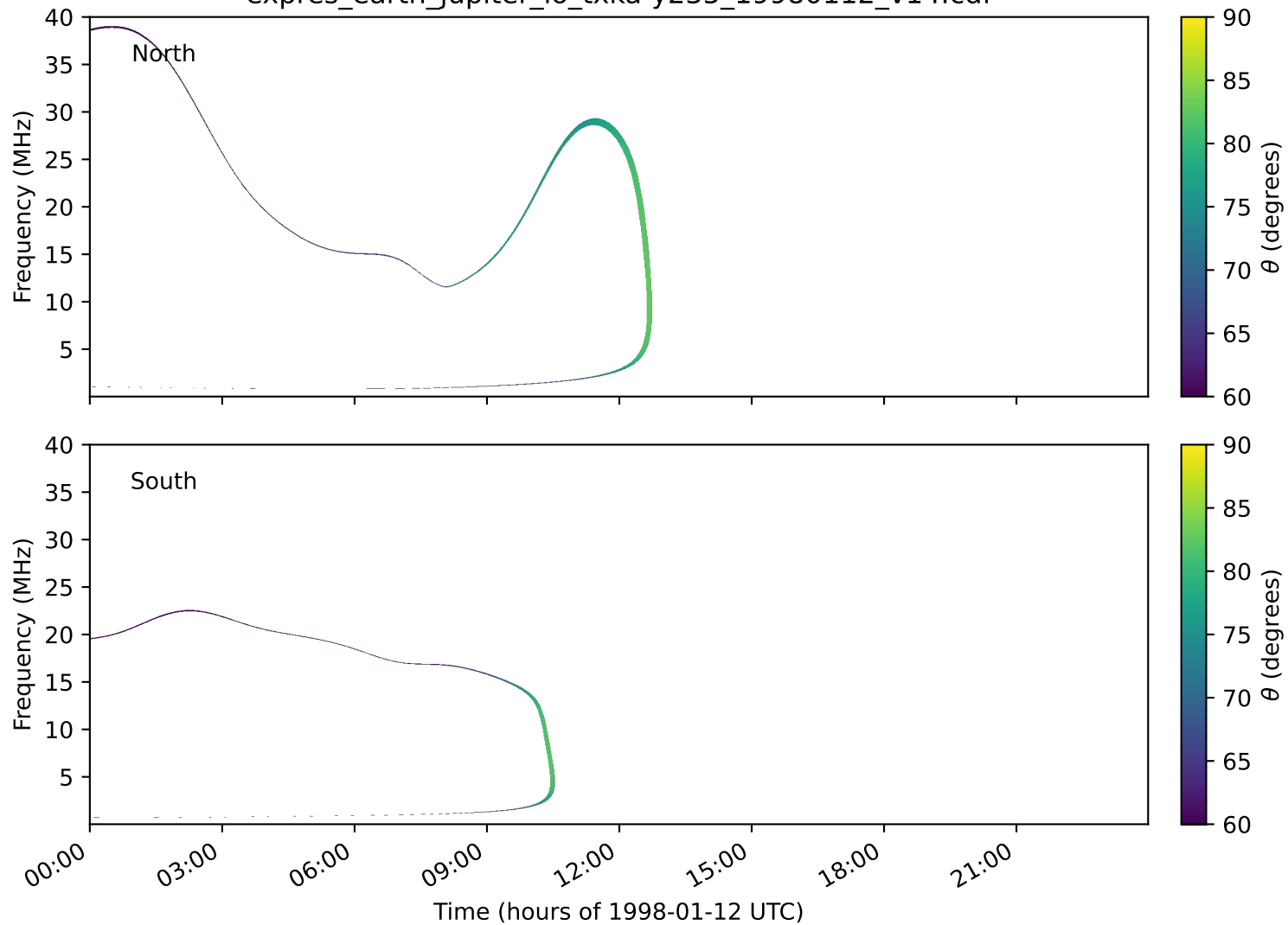
expres_earth_jupiter_io_txka-y235_19980112_v14.cdf
