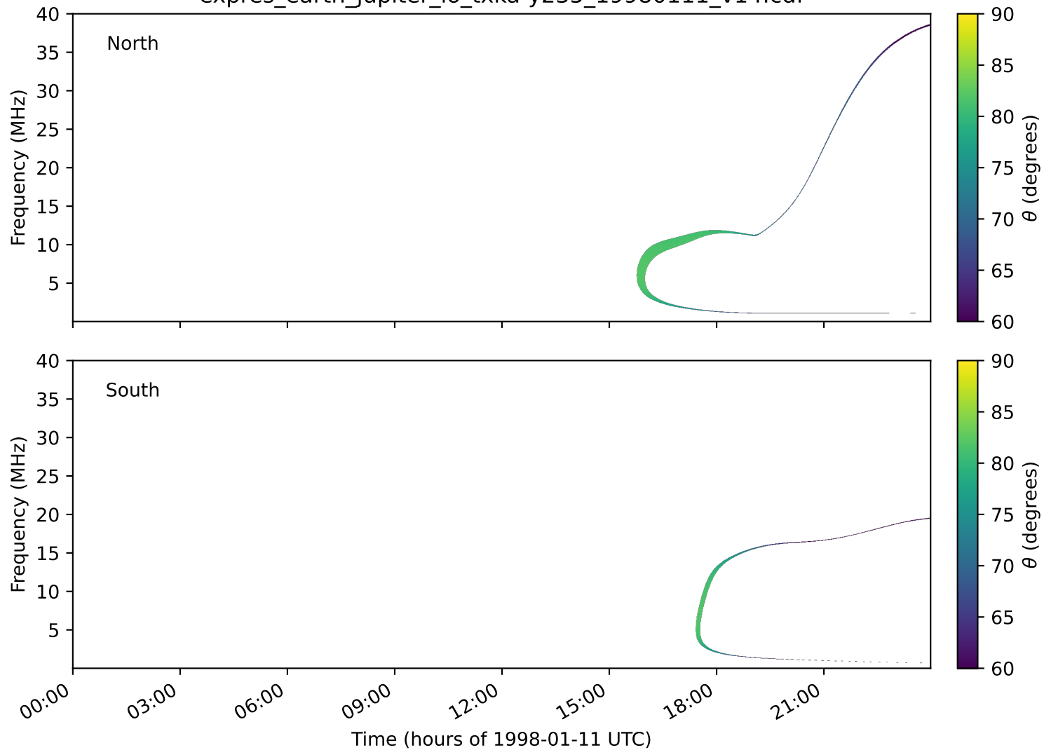
expres_earth_jupiter_io_txka-y235_19980111_v14.cdf
