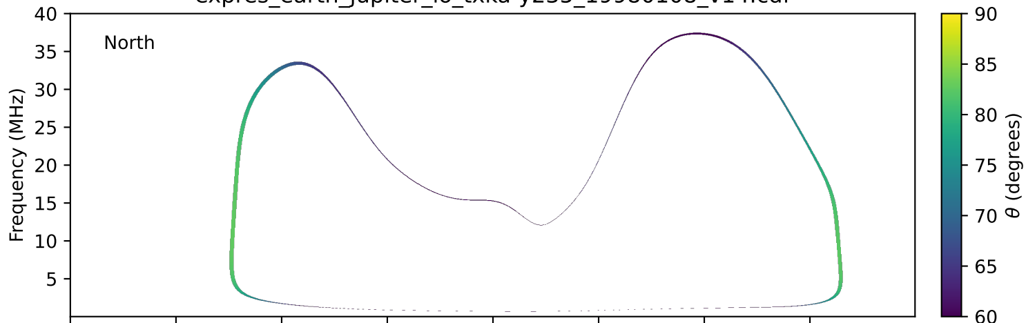
expres_earth_jupiter_io_txka-y235_19980108_v14.cdf
