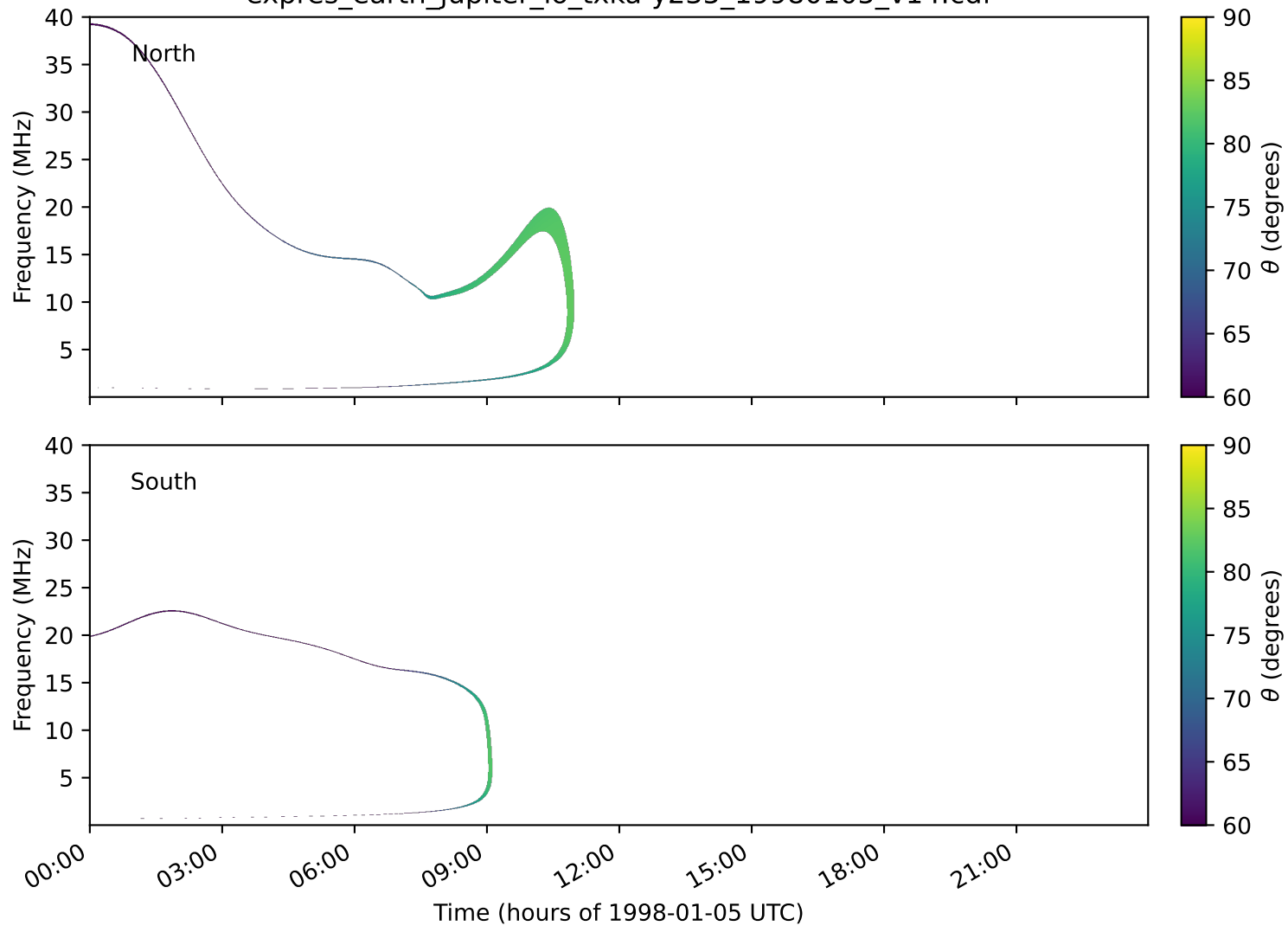
expres_earth_jupiter_io_txka-y235_19980105_v14.cdf
