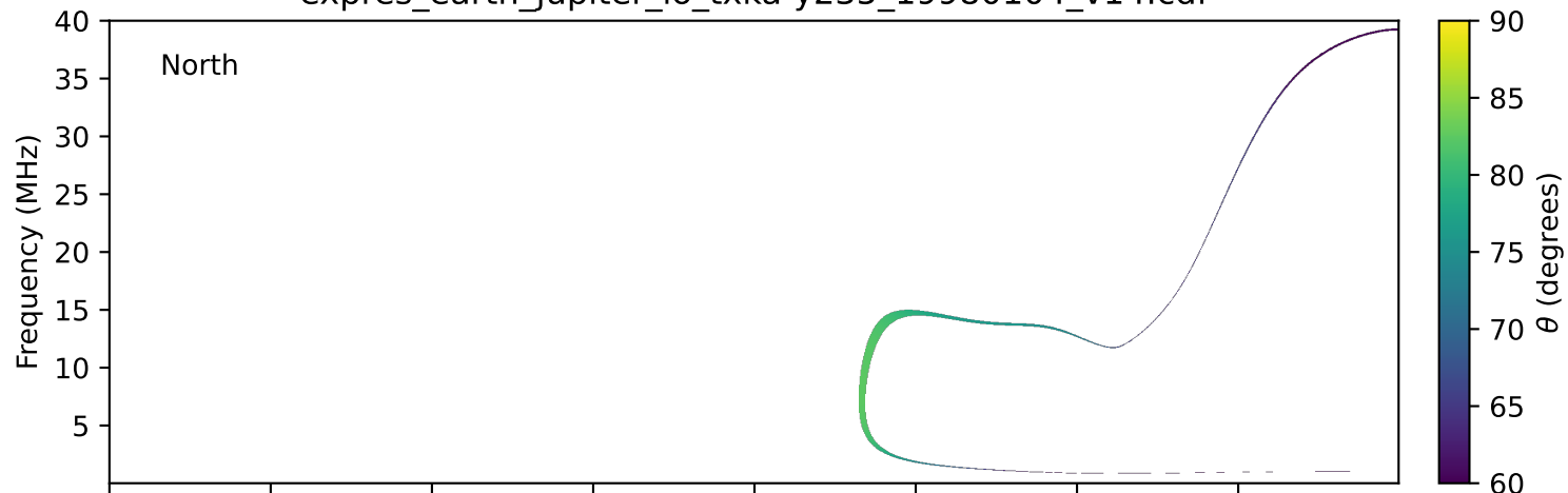
expres_earth_jupiter_io_txka-y235_19980104_v14.cdf
