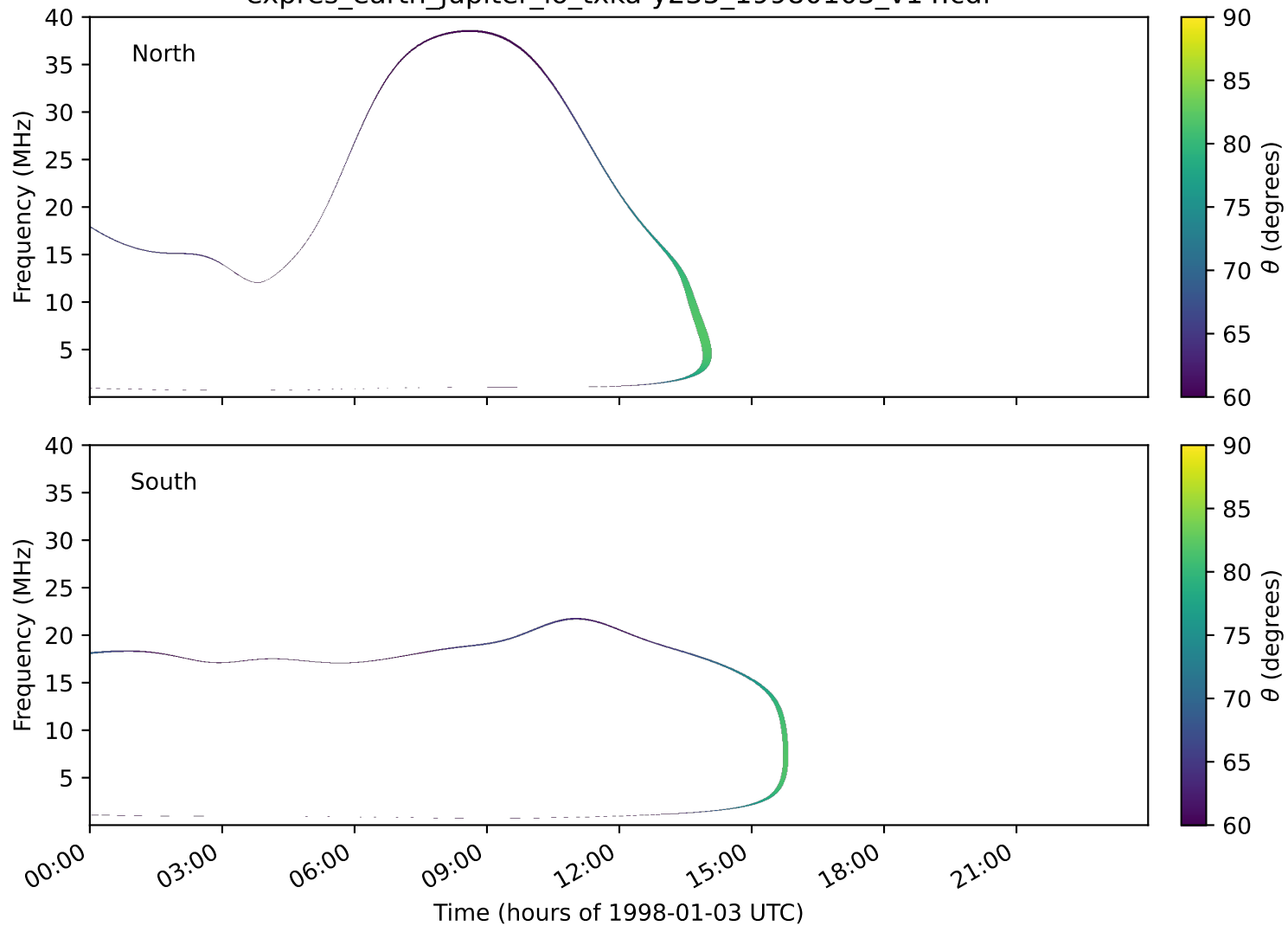
expres_earth_jupiter_io_txka-y235_19980103_v14.cdf
