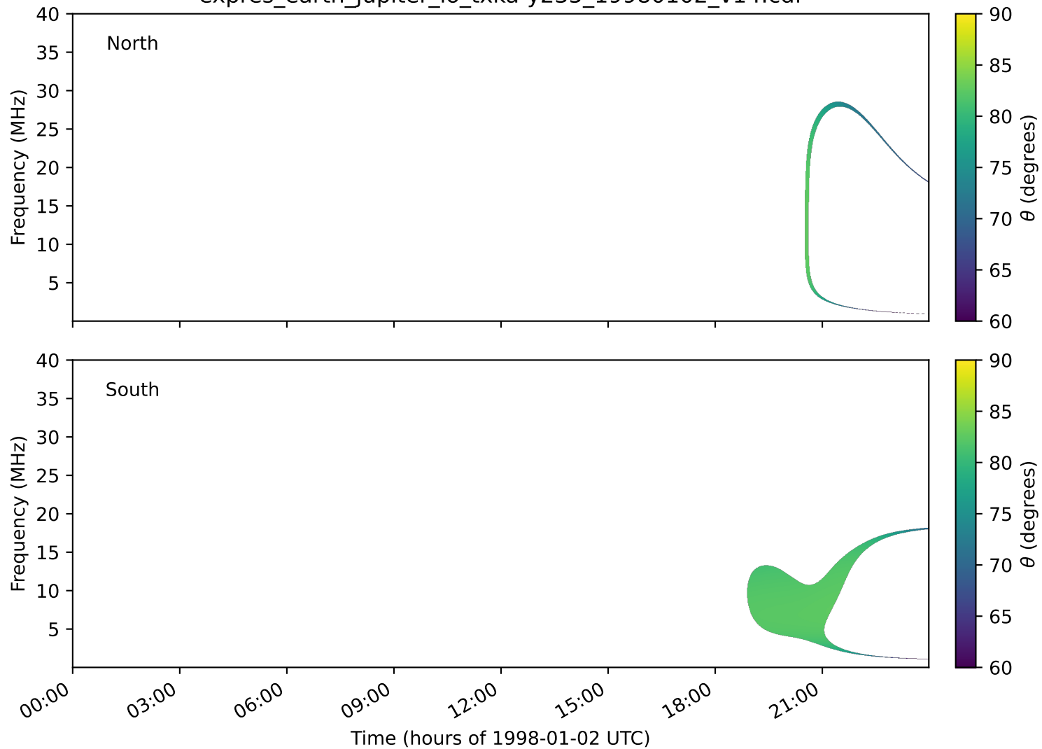
expres_earth_jupiter_io_txka-y235_19980102_v14.cdf
