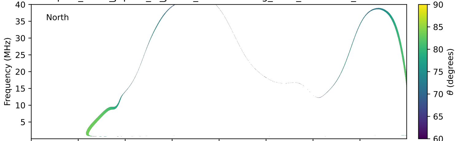
expres_earth_jupiter_io_jrm33_lossc-wid1deg_3kev_19980131_v11.cdf
