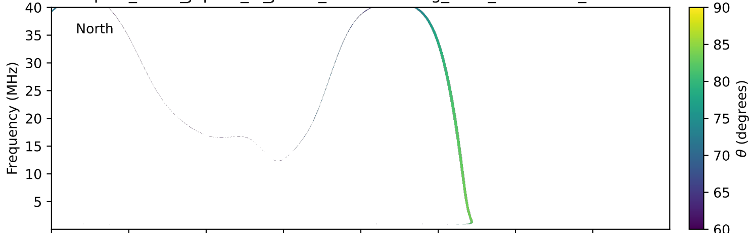
expres_earth_jupiter_io_jrm33_lossc-wid1deg_3kev_19980126_v11.cdf
