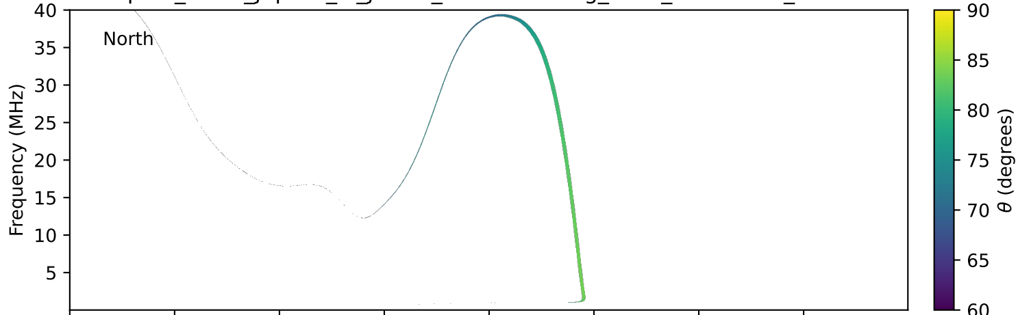
expres_earth_jupiter_io_jrm33_lossc-wid1deg_3kev_19980119_v11.cdf
