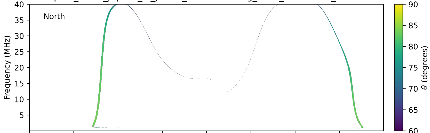
expres_earth_jupiter_io_jrm33_lossc-wid1deg_3kev_19980108_v11.cdf
