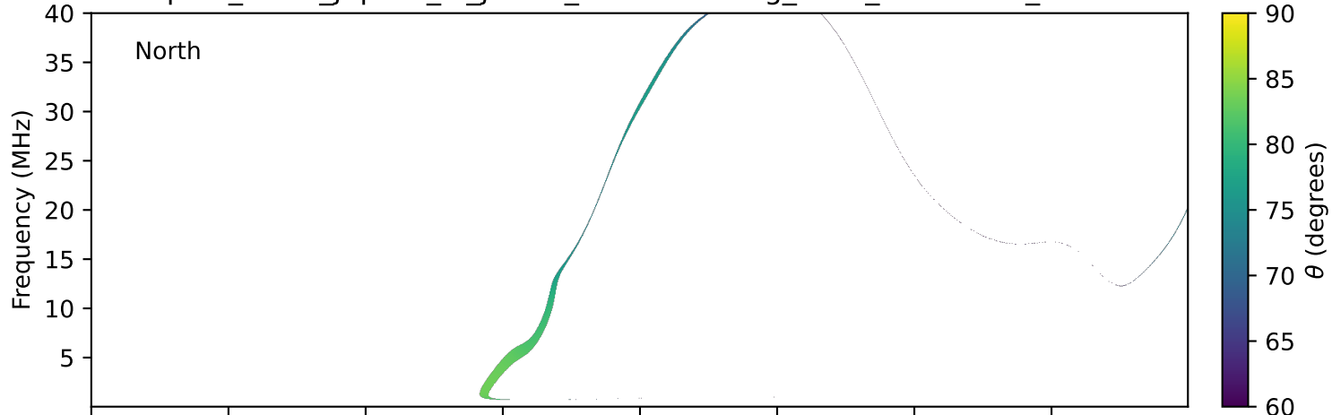
expres_earth_jupiter_io_jrm33_lossc-wid1deg_3kev_19980106_v11.cdf
