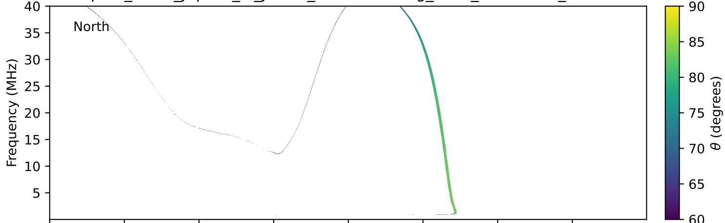
expres_earth_jupiter_io_jrm09_lossc-wid1deg_3kev_19980126_v11.cdf
