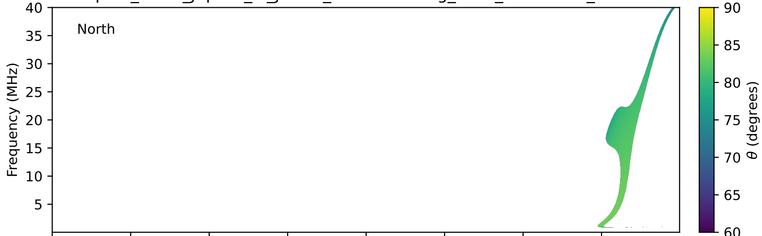
expres_earth_jupiter_io_jrm09_lossc-wid1deg_3kev_19980125_v11.cdf
